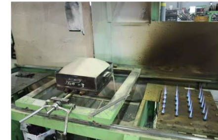
Molding (Coated Sand)
